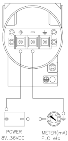
Electrical Connection
